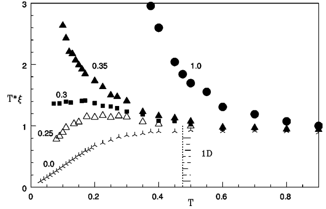
FIG. 3. \xi_y T vs temperature for the two-leg system, when the \alpha 's are close to critical point. Results for \alpha = 0.0 (isolated ladders) and 1.0 (isotropic limit) are added for comparison. The vertical bar indicates the one-dimensional to two-dimensional crossover temperature.
