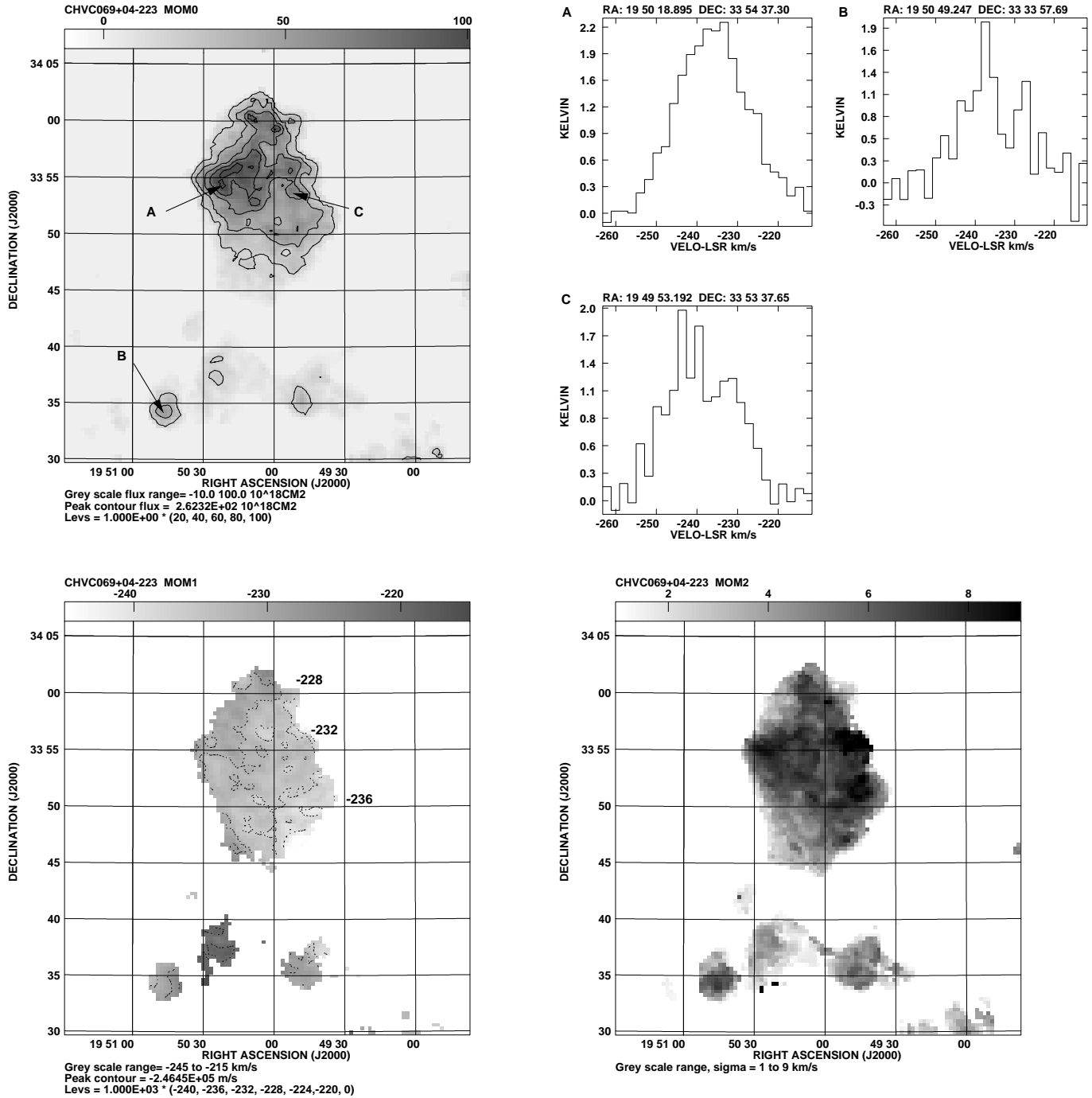
Fig. 1. Imaging data for CHVC 069+04–223 at 1 \text{ arcmin} and 2 \text{ km s}^{-1} resolution. Upper left panel: apparent integrated H I (assuming negligible opacity), with contours at 20, 40, 60, 80, and 100 \times 10^{18} \text{ cm}^{-2} and a linear grey-scale extending from -10 to 100 \times 10^{18} \text{ cm}^{-2} . Upper right panel: brightness temperature spectra at the indicated positions. Lower left panel: intensity weighted line-of-sight velocity, v_{\text{LSR}} , with contours at -240 , -236 , -232 , -228 , -224 , and -220 \text{ km s}^{-1} and a linear grey-scale extending from -245 to -215 \text{ km s}^{-1} . Lower right panel: intensity weighted distribution of squared velocity, corresponding to the velocity dispersion of a Gaussian profile, with a linear grey-scale extending from 1 to 9 \text{ km s}^{-1} .
