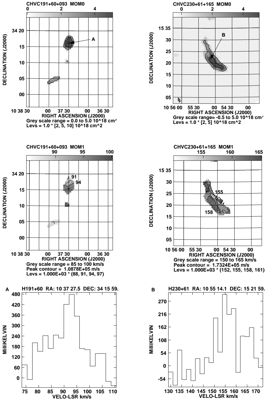
Fig. 10. Imaging data for CHVC 191+60+093 and CHVC 230+61+165 at 2 arcmin and 2 \text{ km s}^{-1} resolution. Upper panels: apparent integrated H I (assuming negligible opacity), with contours at 2, 5, and 10 \times 10^{18} \text{ cm}^{-2} and a linear grey-scale extending from 0 to 5 \times 10^{18} \text{ cm}^{-2} . Middle panels: intensity weighted line-of-sight velocities, v_{\text{LSR}} , with contours at 88, 91, 94, and 97 \text{km s}^{-1} and a linear grey-scale extending from 85 to 100 \text{km s}^{-1} for CHVC 191+60+093, and with contours at 152, 155, 158, and 161 \text{km s}^{-1} and a linear grey-scale extending from 150 to 165 \text{km s}^{-1} for CHVC 230+61+165. Lower panels: brightness temperature spectra at the indicated positions.
