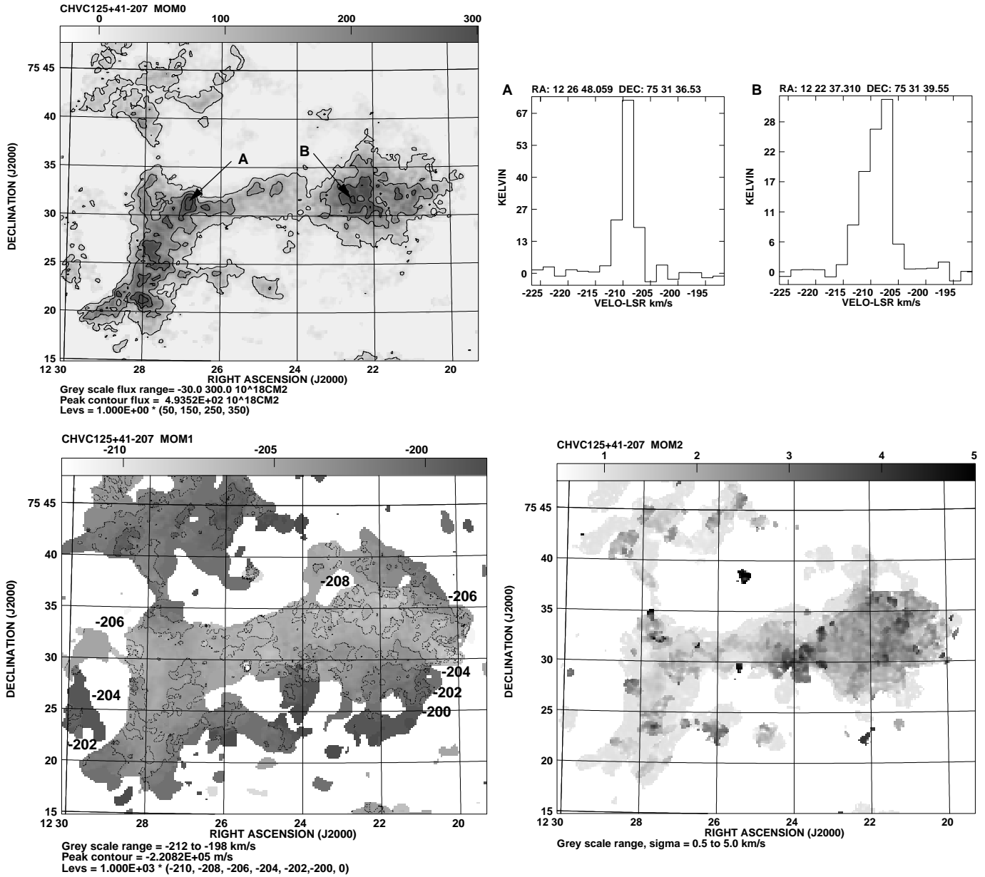
Fig. 5. Imaging data for CHVC 125+41–207 at 28 arcsec and 2 \text{ km s}^{-1} resolution. Upper left panel: apparent integrated H I (assuming negligible opacity), with contours at 50, 150, 250, and 350 \times 10^{18} \text{ cm}^{-2} and a linear grey-scale extending from -30 to 300 \times 10^{18} \text{ cm}^{-2} . Upper right panel: brightness temperature spectra at the indicated positions. The extremely narrow linewidths — the spectrum shown on the left in this panel is one of the narrowest H I emission lines ever observed — robustly constrain the kinetic temperatures. Lower left panel: intensity weighted line-of-sight velocity, v_{\text{LSR}} , with contours at -210 , -208 , -206 , -204 , -202 , and -200 \text{ km s}^{-1} and a linear grey-scale extending from -212 to -198 \text{ km s}^{-1} . Lower right panel: intensity weighted distribution of squared velocity, corresponding to the velocity dispersion of a Gaussian profile, with a linear grey-scale extending from 0.5 to 5 \text{ km s}^{-1} .
