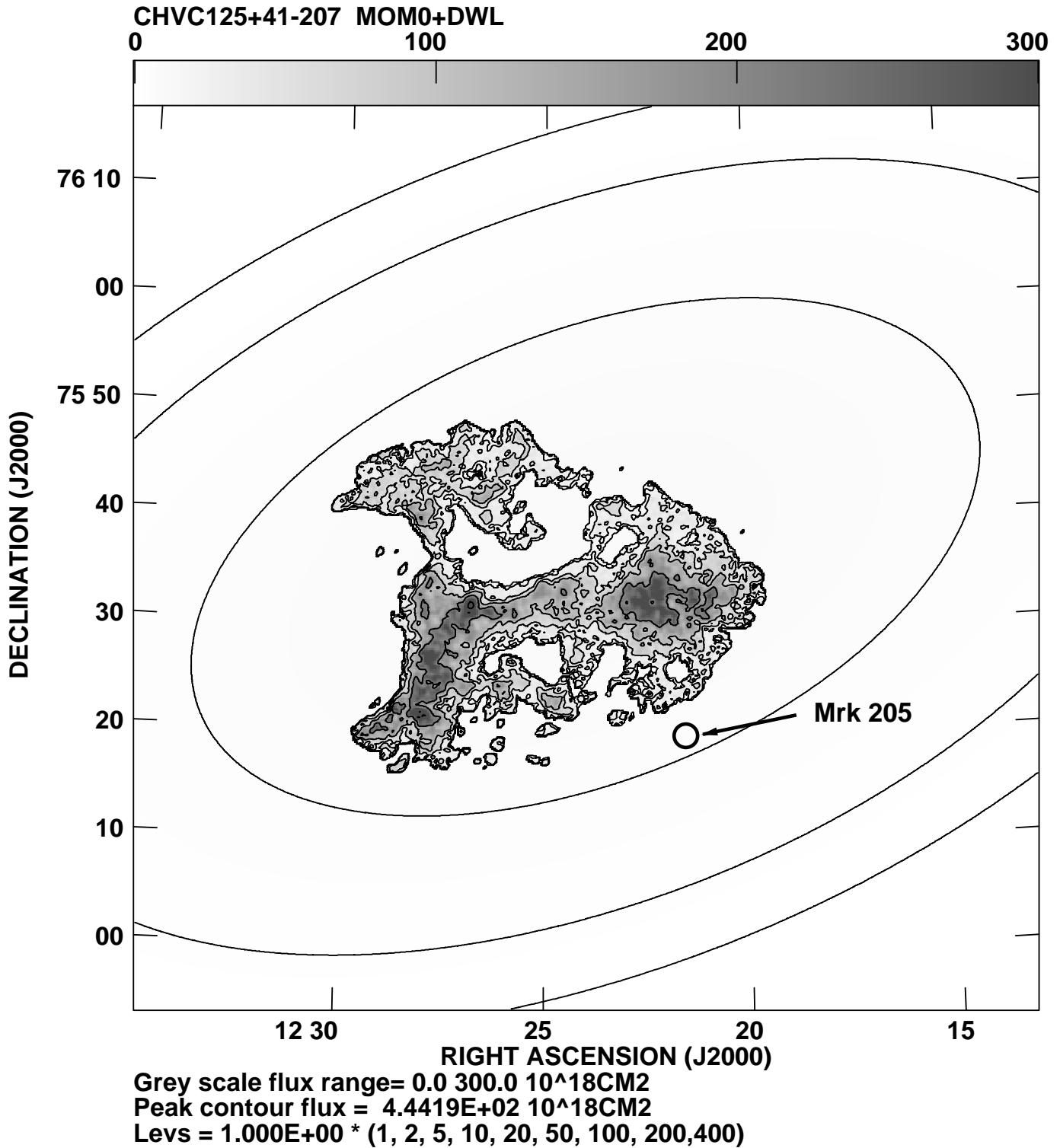
Fig. 7. Column density distribution of H I in CHVC 125+41–207 at 28 arcsec resolution reconstructed from the LDS and WSRT data. Contours are drawn at 1, 2, 5, 10, 20, 50, 100, 200, and 400 \times 10^{18} \text{cm}^{-2} ; a linear grey-scale extends from 0 to 300 \times 10^{18} \text{cm}^{-2} .
