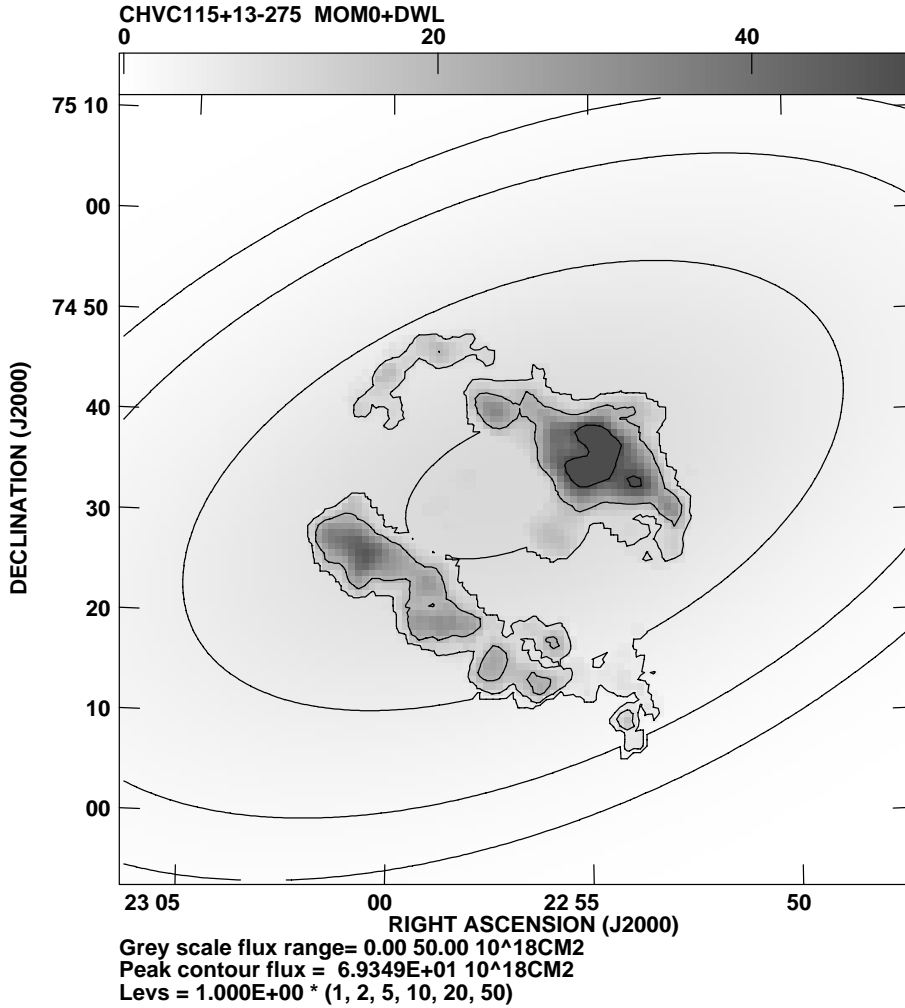
Fig. 4. Column density distribution of H I in CHVC 115+13–275 at 2 arcmin resolution reconstructed using LDS and WSRT data. Contours are drawn at 1, 2, 5, 10, 20, and 50 \times 10^{18} \text{ cm}^{-2} and a linear grey-scale extends from 0 to 50 \times 10^{18} \text{ cm}^{-2} .
