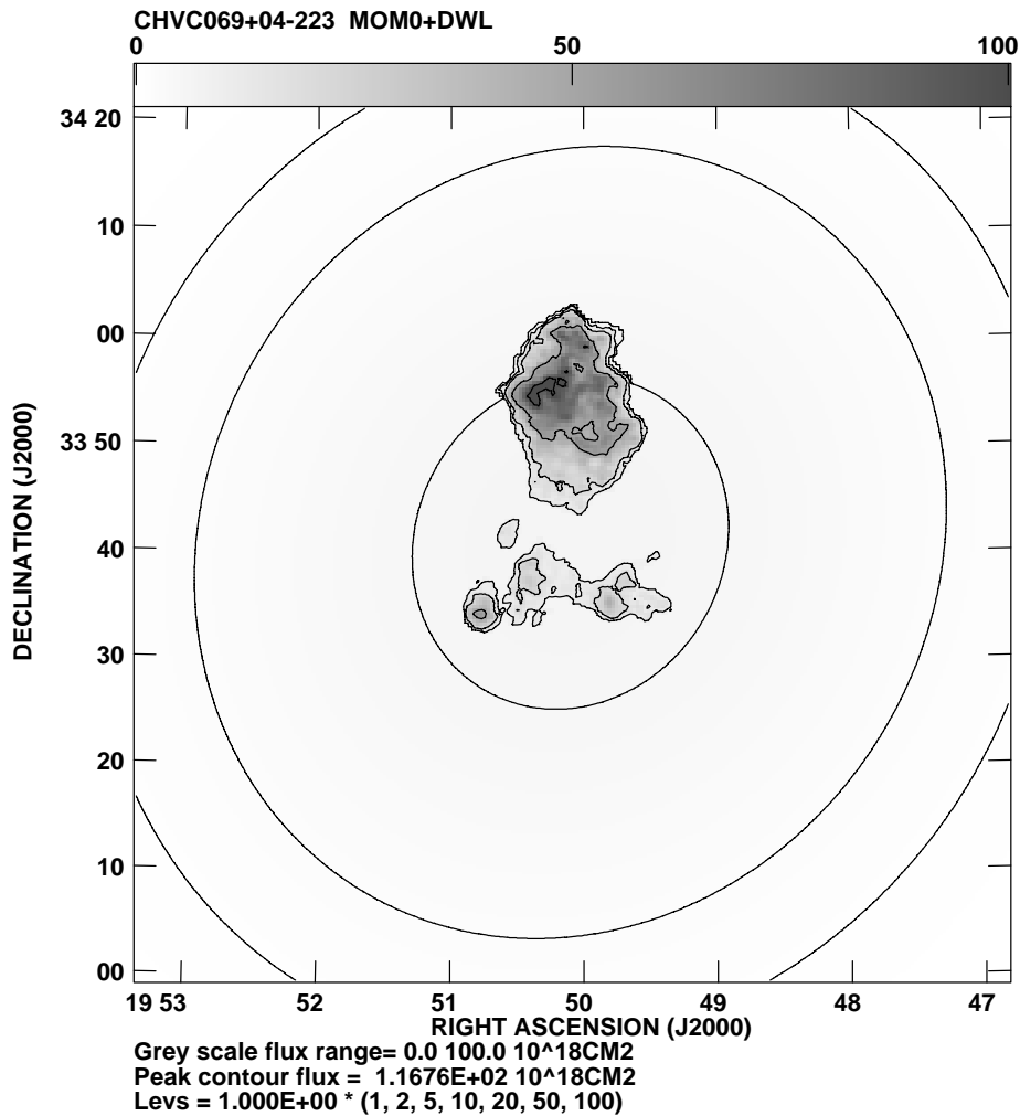
Fig. 2. Column density distribution of H I in CHVC 069+04-223 at 1 arcmin resolution reconstructed from LDS and WSRT data. Contours are drawn at 1, 2, 5, 10, 20, 50, and 100 \times 10^{18} \text{ cm}^{-2} ; a linear grey-scale extends from 0 to 100 \times 10^{18} \text{ cm}^{-2} .
