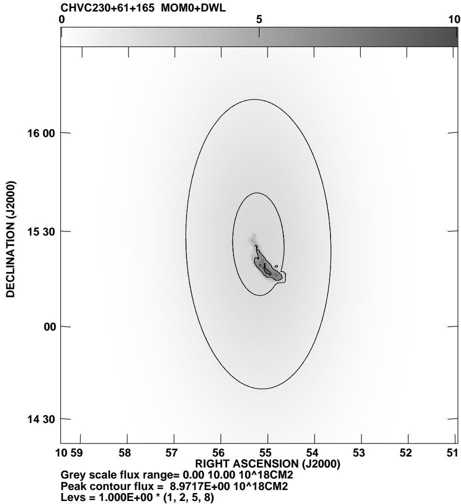
Fig. 12. Column density distribution of H I in CHVC 230+61+165 at 2 arcmin resolution reconstructed from LDS and WSRT data. Contours are drawn at 1, 2, 5, and 8 \times 10^{18} \text{ cm}^{-2} and a linear grey-scale extends from 0 to 10 \times 10^{18} \text{ cm}^{-2} .
