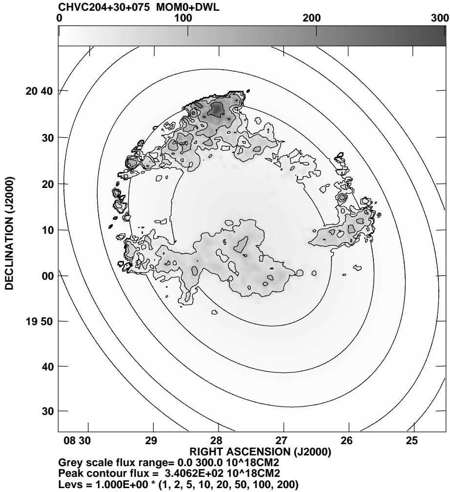
Fig. 9. Column density distribution of H I in CHVC 204+30+075 at 1 arcmin resolution reconstructed from LDS and WSRT data. Contours are drawn at 1, 2, 5, 10, 20, 50, 100, and 200 \times 10^{18} \text{ cm}^{-2} ; a linear grey-scale extends from 0 to 300 \times 10^{18} \text{ cm}^{-2} .
