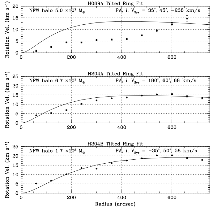
Fig. 14. Derived rotation velocities in three elliptical cores, CHVC 069+04–223A and CHVC 204+30+075A and B. The best-fitting position angle, inclination, and systemic velocity are indicated at the top right of each panel. These were subsequently held fixed in deriving the rotation velocity as function of radius. Solid lines are the rotation curves of NFW cold dark matter halos of the indicated mass.
