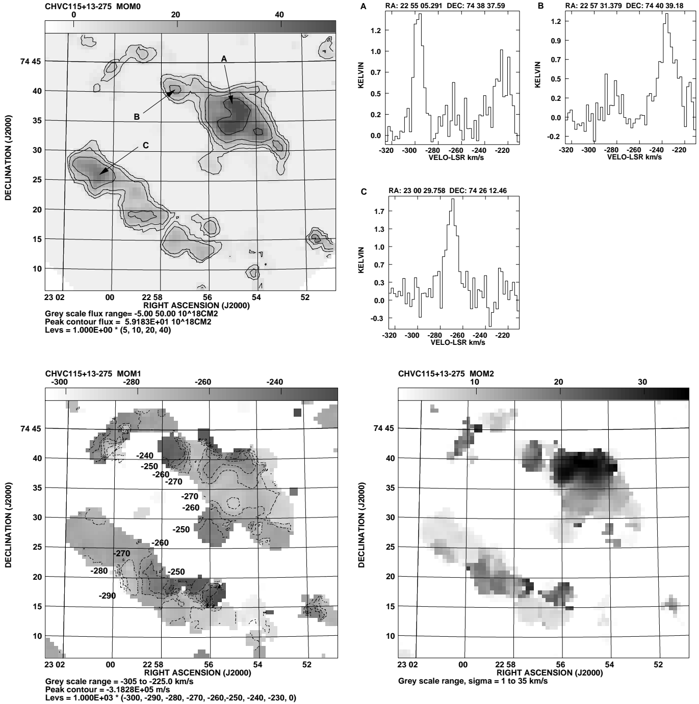
Fig. 3. Imaging data for CHVC 115+13–275 at 2 arcmin and 2 \text{ km s}^{-1} resolution. Upper left panel: apparent integrated HI (assuming negligible opacity), with contours at 5, 10, 20, and 40 \times 10^{18} \text{ cm}^{-2} and a linear grey-scale extending from -5 to 50 \times 10^{18} \text{ cm}^{-2} . Upper right panel: brightness temperature spectra at the indicated positions. Lower left panel: intensity weighted line-of-sight velocity, v_{\text{LSR}} , with contours at -300 to -230 \text{ km s}^{-1} in steps of 10 \text{ km s}^{-1} and a linear grey-scale extending from -305 to -225 \text{ km s}^{-1} . Lower right panel: intensity weighted distribution of squared velocity, corresponding to the velocity dispersion of a Gaussian profile, with a linear grey-scale extending from 1 to 35 \text{ km s}^{-1} .
