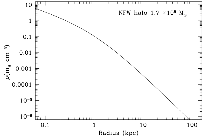
Fig. 15. Mass volume density, in units of hydrogen nuclei per cubic centimeter, as a function of radius for an NFW cold dark matter halo of mass 10^{8.2} M_{\odot} within the 12.6 kpc virial radius.
