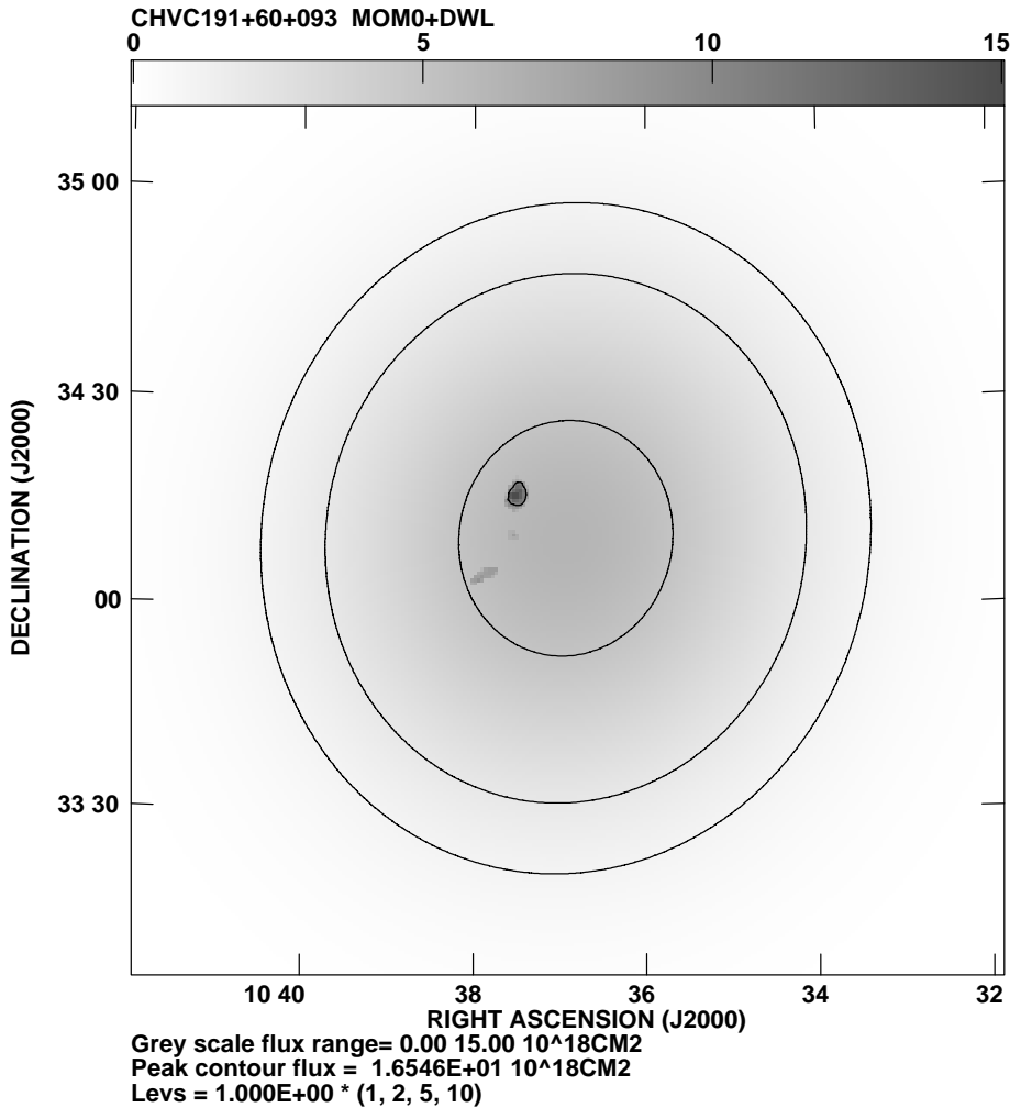
Fig. 11. Column density distribution of HI in CHVC 191+60+093 at 2 arcmin resolution reconstructed using LDS and WSRT data. Contours are drawn at 1, 2, 5, and 10 \times 10^{18} \text{ cm}^{-2} and a linear grey-scale extends from 0 to 15 \times 10^{18} \text{ cm}^{-2} .
