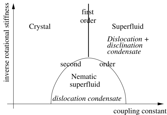
Fig. 5. The generic phase diagram associated with 2 + 1D Bosonic matter, assuming that the field theoretic description based on quantum elasticity is of relevance. When the rotational stiffness is small a first order transition from the crystal directly into the superfluid is expected, corresponding with a simultaneous Bose condensation of dislocations and disclinations (or better condensation of 'defects'). Upon increasing the rotational stiffness, disclinations become expensive and at intermediate coupling constants a dislocation-only condensate will emerge. These are the nematic superfluids which are at the focus of this paper.
