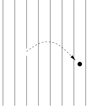
Fig. 2. Individual atoms can leave their equilibrium positions, leaving behind a vacancy-interstitial pair, called in this paper ‘interstitial.’ These point-like defects cannot be avoided at any finite temperature while at zero temperature their condensation causes the supersolid. As in other pictures, the lines just refer to ‘rows of atoms.’
