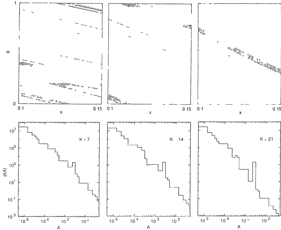
FIG 3 (Color online) Upper panels: phase space portrait of lead 1, for \tau_D=10 and different values of K . Each point represents an initial condition for the classical map (2.4), which is either transmitted through lead 2 (black/red) or reflected back through lead 1 (gray/green). Only initial conditions with dwell times \leq 3 are shown for clarity. Lower panels: histogram of the area distribution of the transmission and reflection bands, calculated from the corresponding phase-space portrait in the upper panel. Areas greater than h_{\text{eff}}=1/M correspond to noiseless scattering channels.
