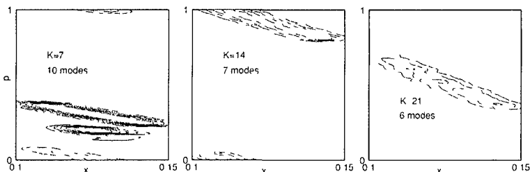
FIG. 4. (Color online) Contour plots of the Husimi function (5.3) in lead 1 for M = 2400 , \tau_D = 10 , and K = 7, 14, 21 . The outer contour is at the value 0.15, inner contours increase with increments of 0.1. Yellow regions are the classical transmission bands with area > 1/M , extracted from Fig. 3.
