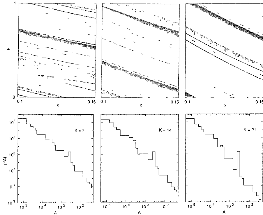
FIG. 3 (Color online) Upper panels: phase-space portrait of lead 1, for \tau_D = 10 and different values of K . Each point represents an initial condition for the classical map (2.4), which is either transmitted through lead 2 (black/red) or reflected back through lead 1 (gray/green). Only initial conditions with dwell times \leq 3 are shown for clarity. Lower panels: histogram of the area distribution of the transmission and reflection bands, calculated from the corresponding phase-space portrait in the upper panel. Areas greater than h_{\text{eff}} = 1/M correspond to noiseless scattering channels.
