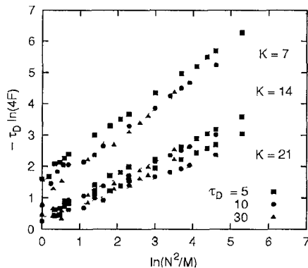
FIG 2 Demonstration of the logarithmic scaling of the Fano factor F with the parameter N^2/M=M/(2\tau_D)^2 . The data points follow from the quantum mechanical simulation and the lines are the analytical prediction (3.1), with c being a fit parameter. The slope \lambda^{-1}=1/\ln(K/2) of each line is not a fit parameter.
