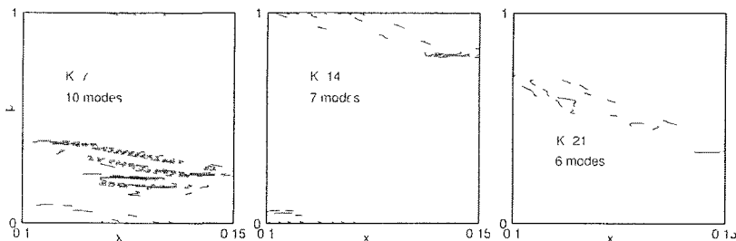
FIG 4 (Color online) Contour plots of the Husimi function (5.3) in lead 1 for M=2400 , \tau_D=10 , and K=7, 14, 21 . The outer contour is at the value 0.15; inner contours increase with increments of 0.1. Yellow regions are the classical transmission bands with area > 1/M extracted from Fig. 3.
