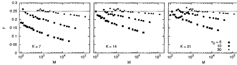
FIG 1 Dependence of the Fano factor F on the dimensionality of the Hilbert space M=1/h_{\text{eff}} , at fixed dwell time \tau_D=M/2N and kicking strength K . The data points follow from the quantum-mechanical simulation in the open kicked rotator. The solid line at F=1/4 is the M -independent result of random matrix theory. The dashed lines are the semiclassical calculation using the theory of Ref. 5. There are no fit parameters in the comparison between theory and simulation.
