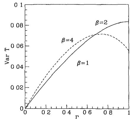
FIG. 2. Variance of the transmission probability T as a function of the transmission probability of the leads \Gamma .
