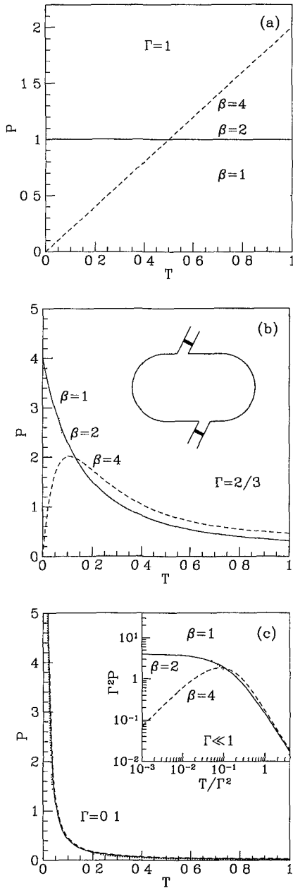
FIG. 1. Distribution of the transmission probability T through a quantum dot with nonideal single-channel leads, for three values of the transmission probability \Gamma of the leads. The curves are computed from Eq. (11) for each symmetry class ( \beta=1,2,4 ). The inset of (b) shows the quantum dot, the inset of (c) shows the asymptotic behavior of P(T) for \Gamma \ll 1 on a log-log scale.
