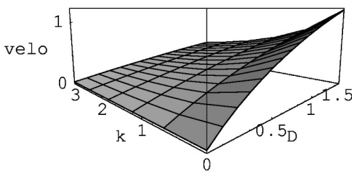
FIG. 1. The front velocity as a function of D and k , as determined from the analysis in Sec. II.
