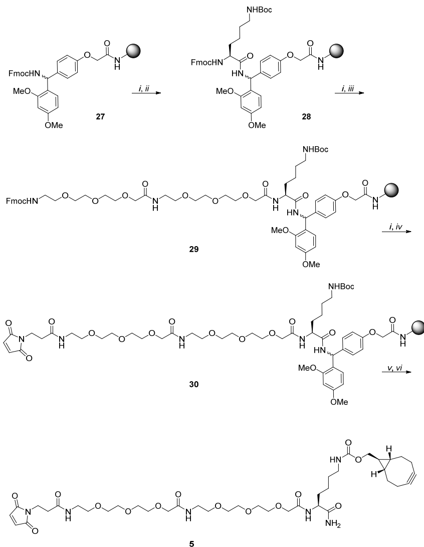
Scheme 5. Reagents and conditions: (i) piperidine, DMF, rt, 20 min (ii) Fmoc-Lys(Boc)-OH, HCTU, DIPEA, DMF, rt, 1 hr (iii) 10, HCTU, DIPEA, DMF, rt, 1 hr (iv) 3-maleimidopropionic acid NHS ester, DIPEA, DMF, rt, 4 hrs (v) TFA – H 2 O – TIPS (190:5:5), rt, 3 hrs (vi) 9, DIPEA, DMF, rt, 4 hrs, 25%.
