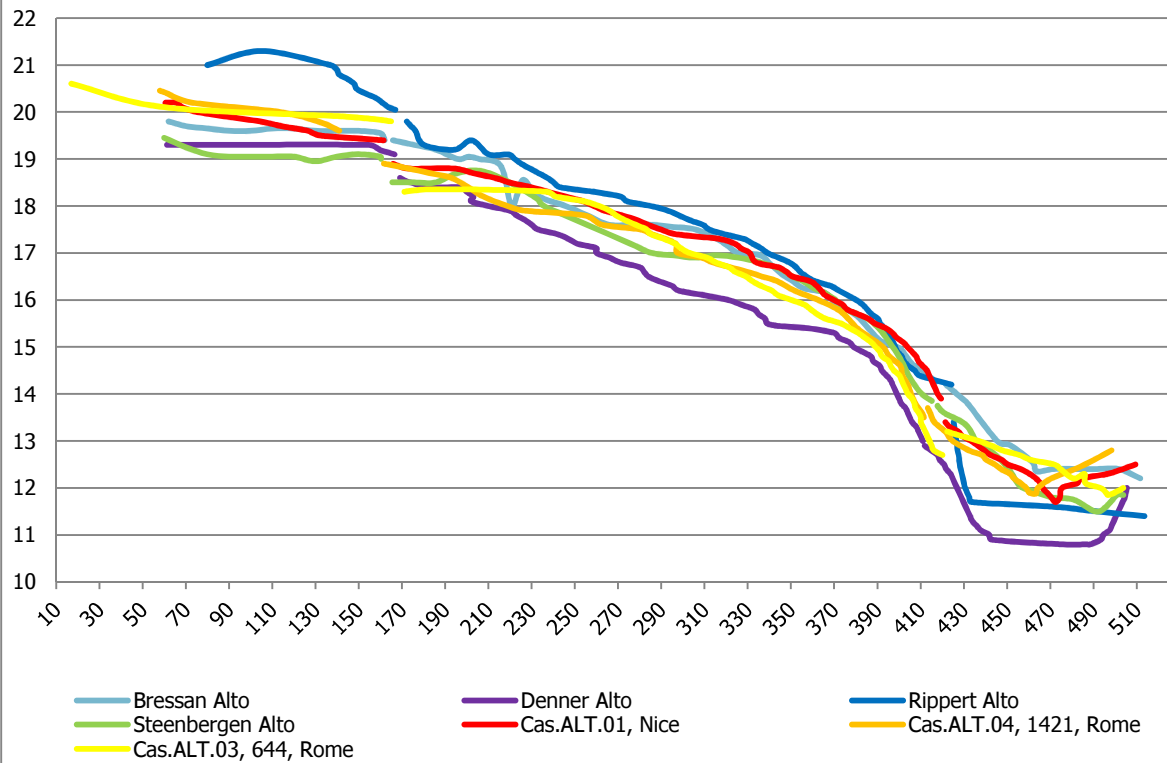
Chart 1.5.17: Bore profiles of Castel, Bressan, Denner, Rippert and Steenberg alto
