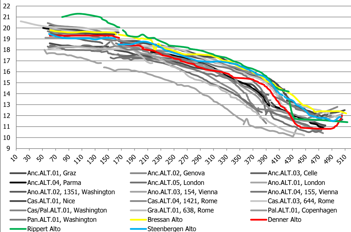
1.5.18a: Chart of studied altos with Bressan, Denner, Rippert and Steenberg
